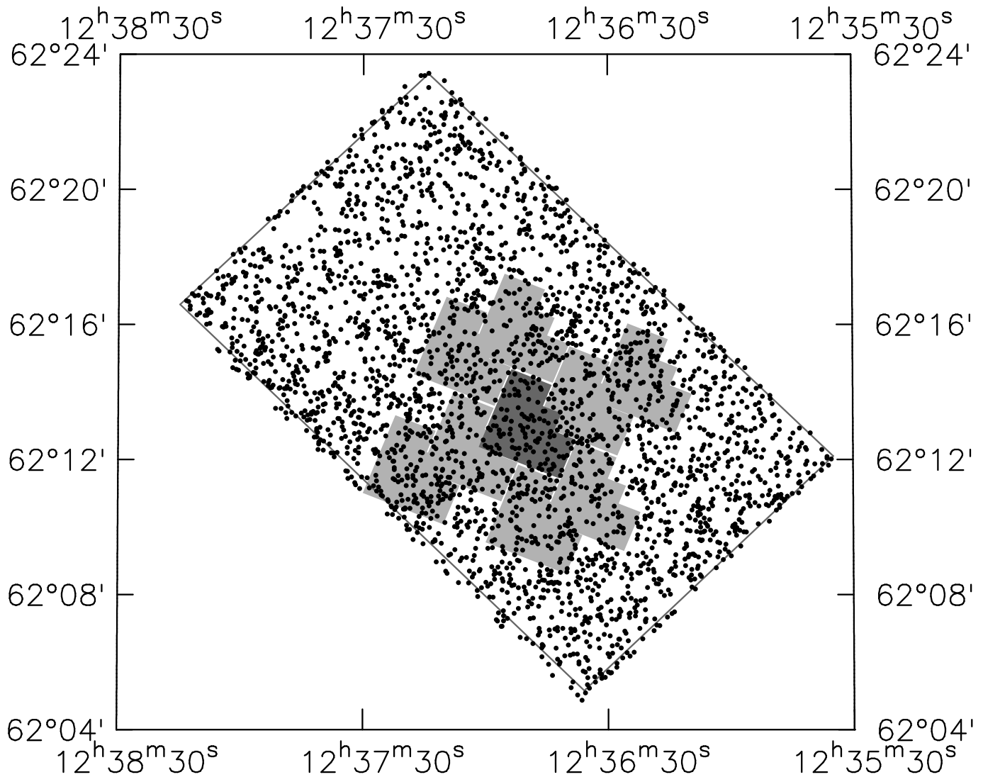
FIG. 3.— Projected sky distribution of objects in the DEIMOS spectroscopic survey sample. Shaded areas indicate the Hubble Deep Field ( dark grey ) and the flanking fields ( light grey ). The outline indicates approximately the first-epoch HST ACS GOODS-N imaging survey region.
